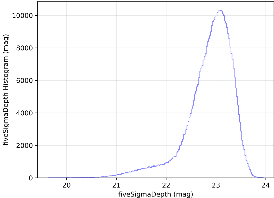
internal_u_expt30_nscale1.1v3.4_10yrs All sky z band: fiveSigmaDepth Histogram
