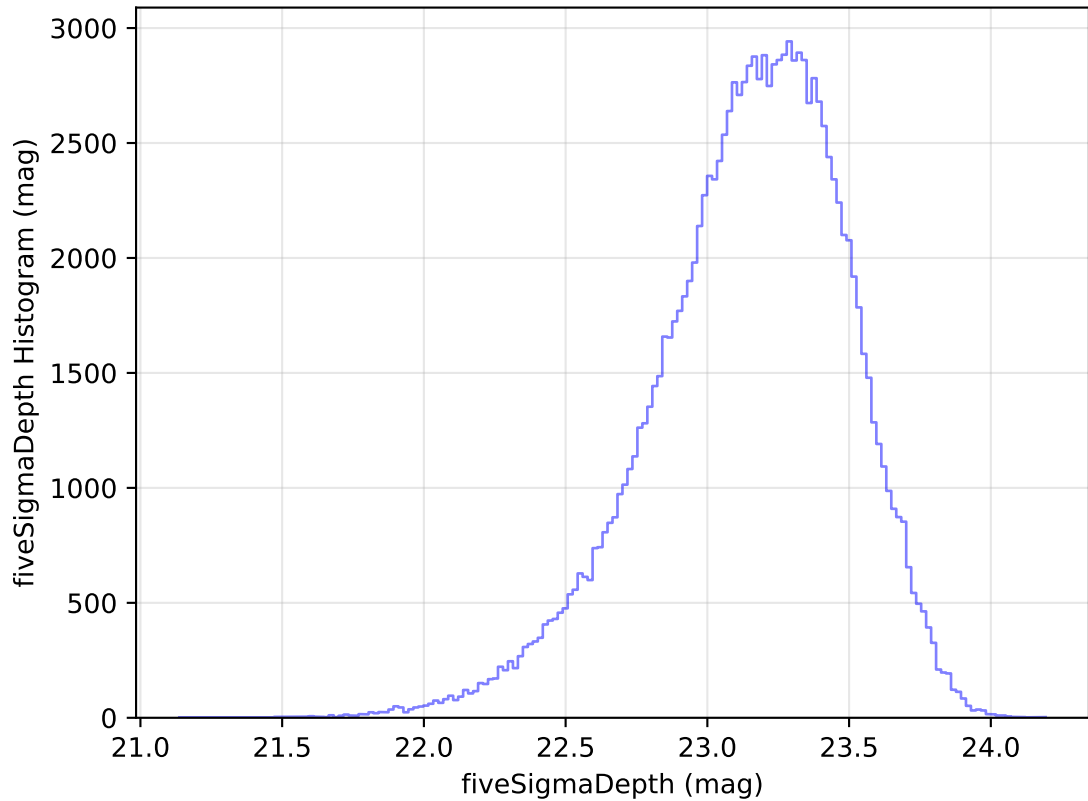
internal_u_expt30_nscale1.1v3.4_10yrs All sky u band: fiveSigmaDepth Histogram
