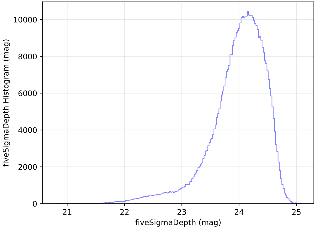
internal_u_expt30_nscale1.1v3.4_10yrs All sky r band: fiveSigmaDepth Histogram
