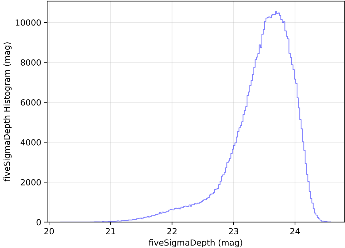
internal_u_expt30_nscale1.1v3.4_10yrs All sky i band: fiveSigmaDepth Histogram
