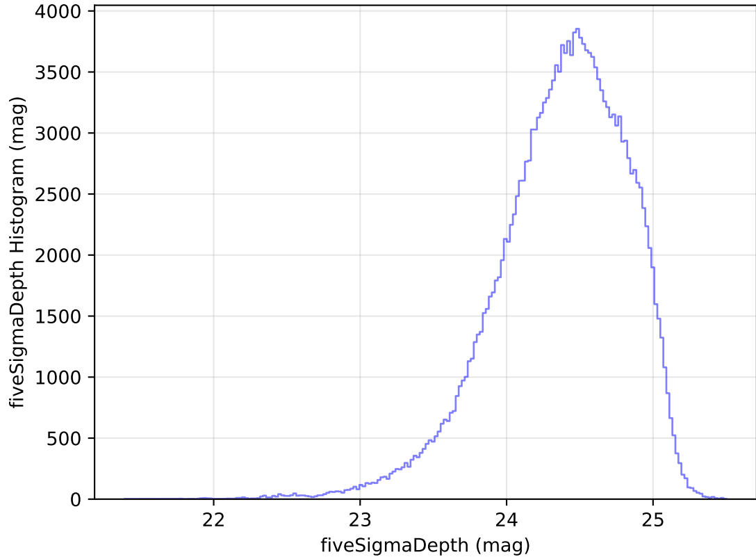
internal_u_expt30_nscale1.1v3.4_10yrs All sky g band: fiveSigmaDepth Histogram
