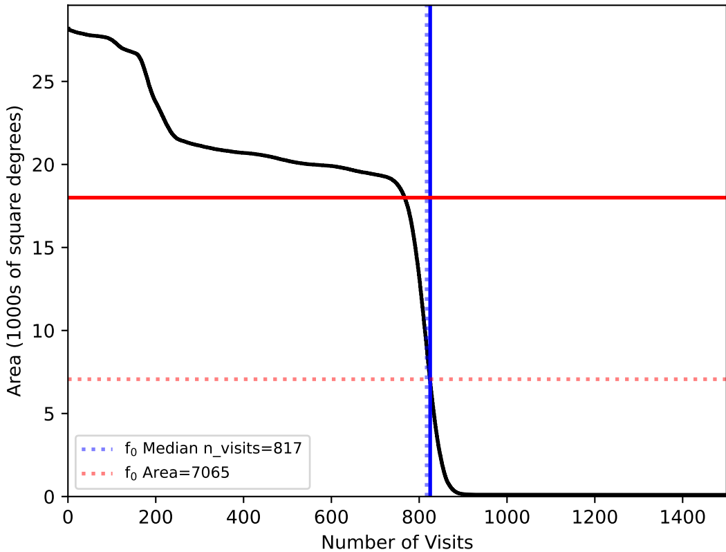
internal_u_expt30_nscale1.1v3.4_10yrs All sky: f0
