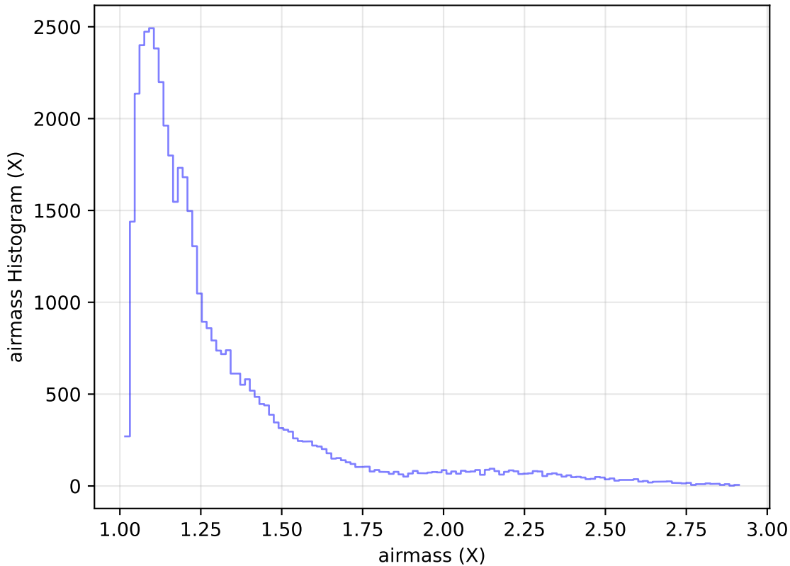
internal_u_expt30_nscale1.1v3.4_10yrs Yr 1 z band: airmass Histogram
