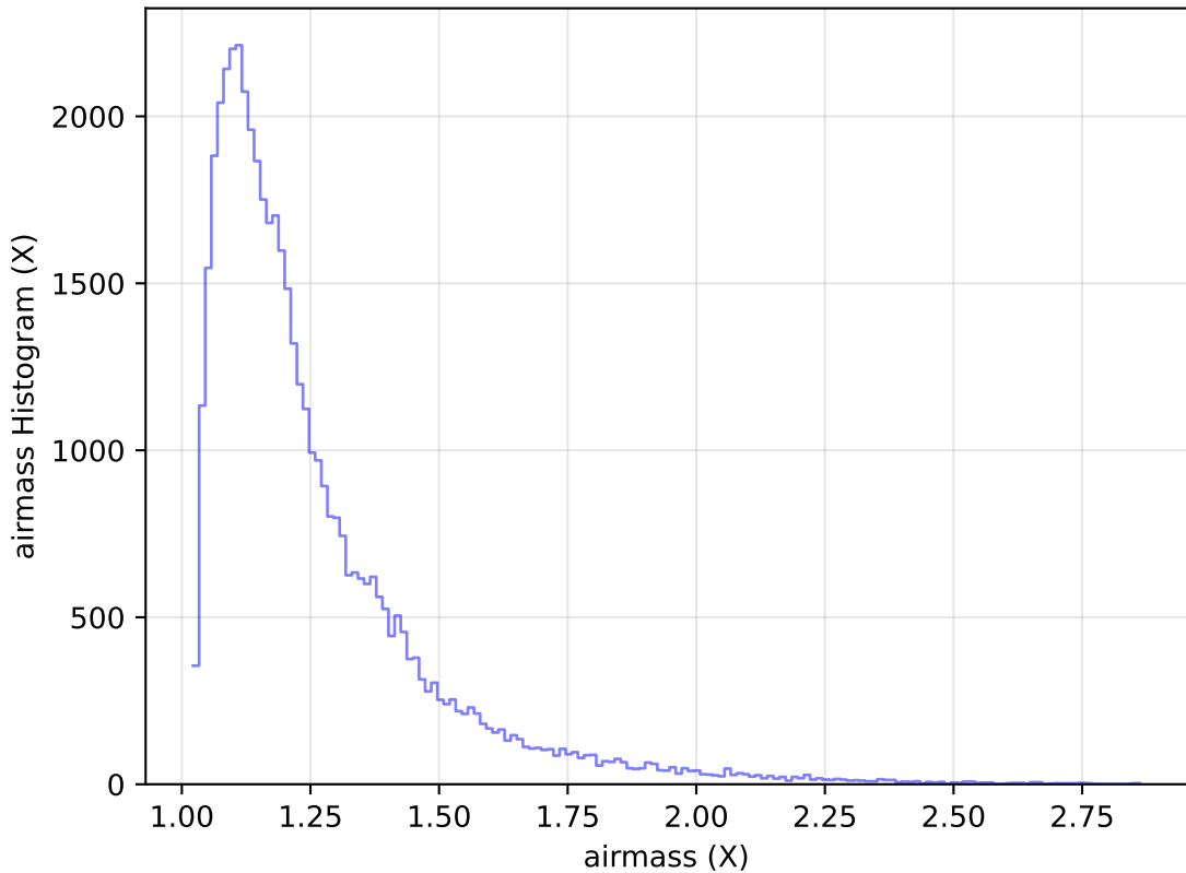
internal_u_expt30_nscale1.1v3.4_10yrs Yr 1 y band: airmass Histogram
