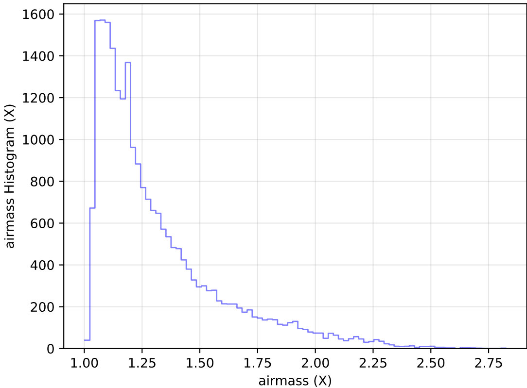
internal_u_expt30_nscale1.1v3.4_10yrs Yr 1 g band: airmass Histogram
