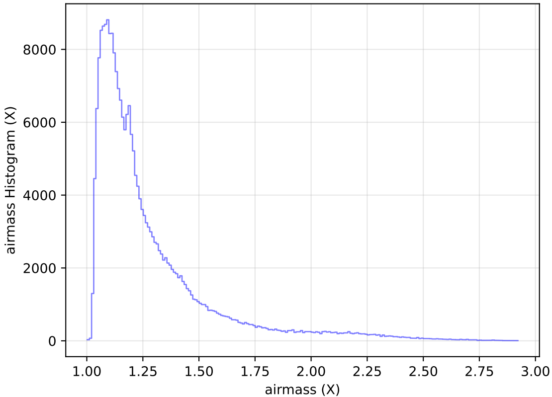
internal_u_expt30_nscale1.1v3.4_10yrs Yr 1 all bands: airmass Histogram
