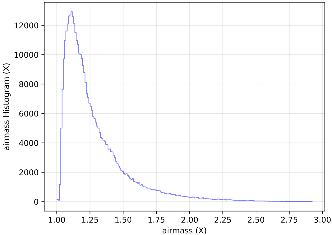
internal_u_expt30_nscale1.1v3.4_10yrs WFD y band: airmass Histogram
