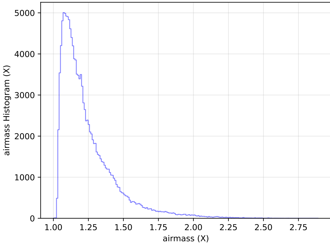
internal_u_expt30_nscale1.1v3.4_10yrs WFD u band: airmass Histogram
