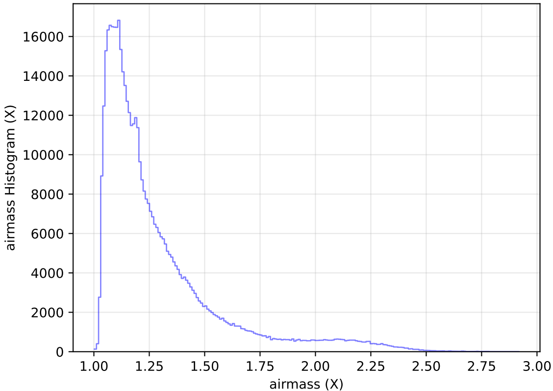
internal_u_expt30_nscale1.1v3.4_10yrs WFD r band: airmass Histogram
