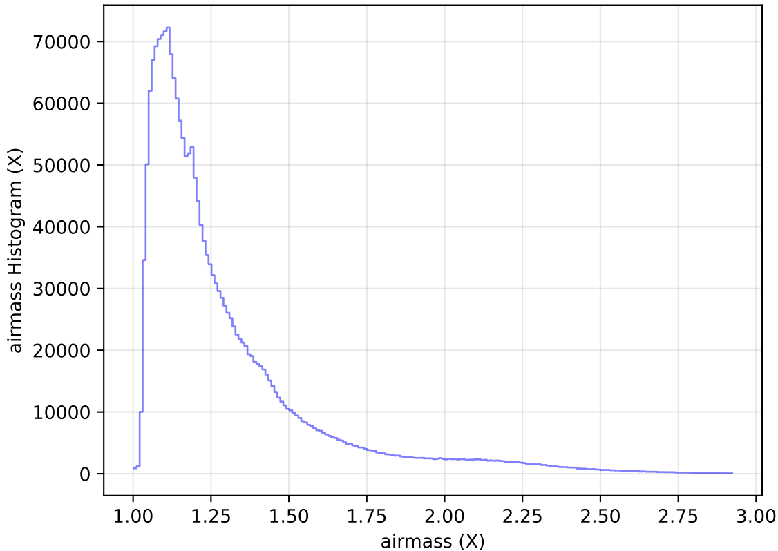
internal_u_expt30_nscale1.1v3.4_10yrs WFD all bands: airmass Histogram
