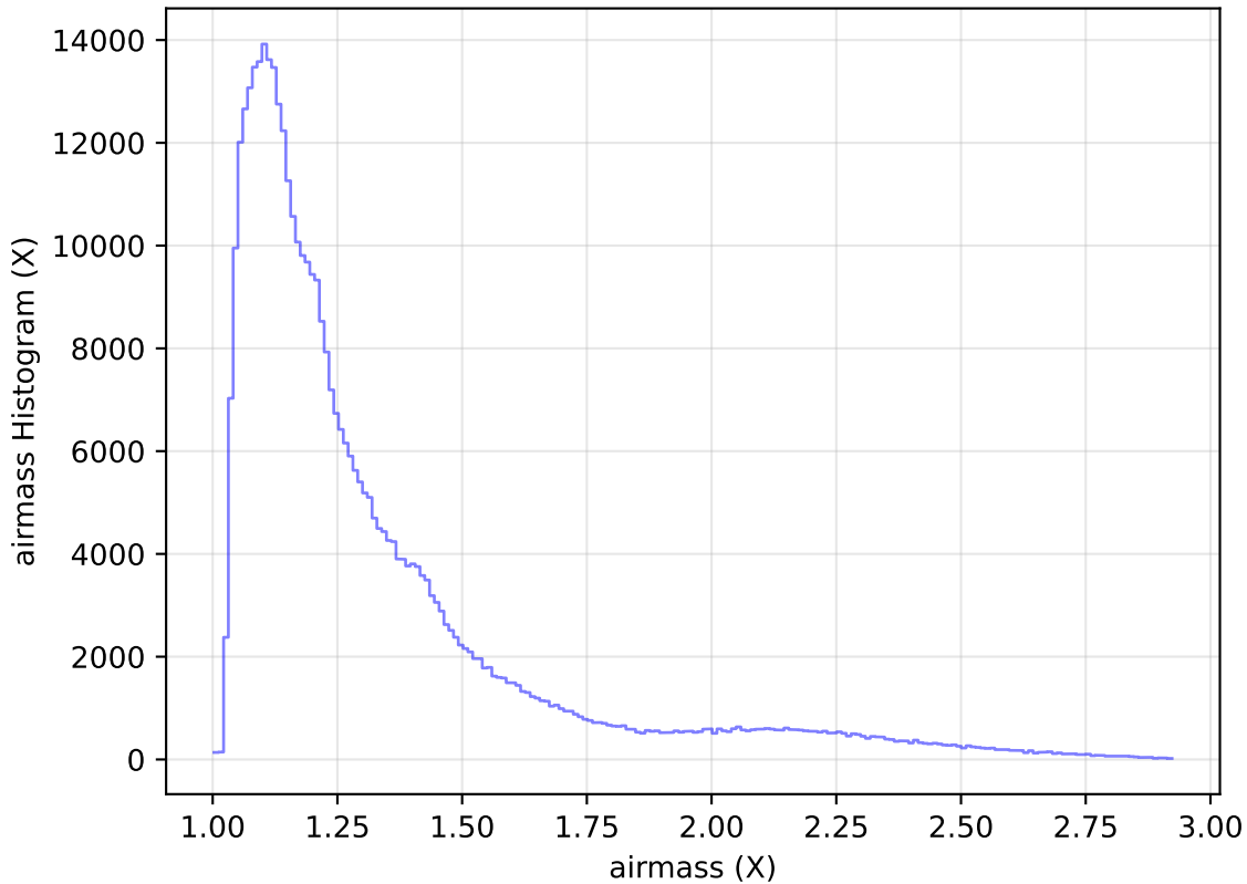
internal_u_expt30_nscale1.1v3.4_10yrs All sky z band: airmass Histogram
