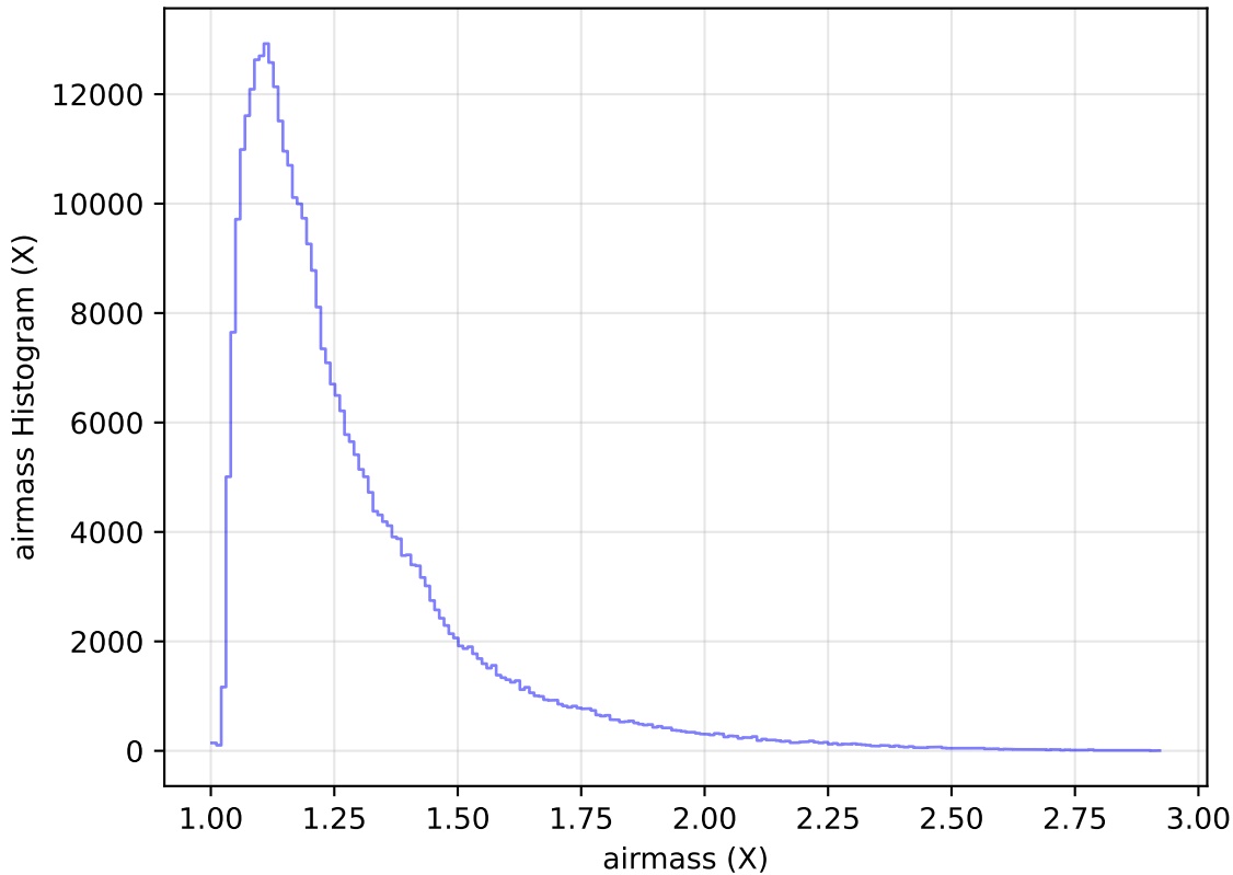
internal_u_expt30_nscale1.1v3.4_10yrs All sky y band: airmass Histogram
