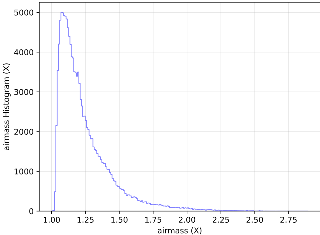
internal_u_expt30_nscale1.1v3.4_10yrs All sky u band: airmass Histogram
