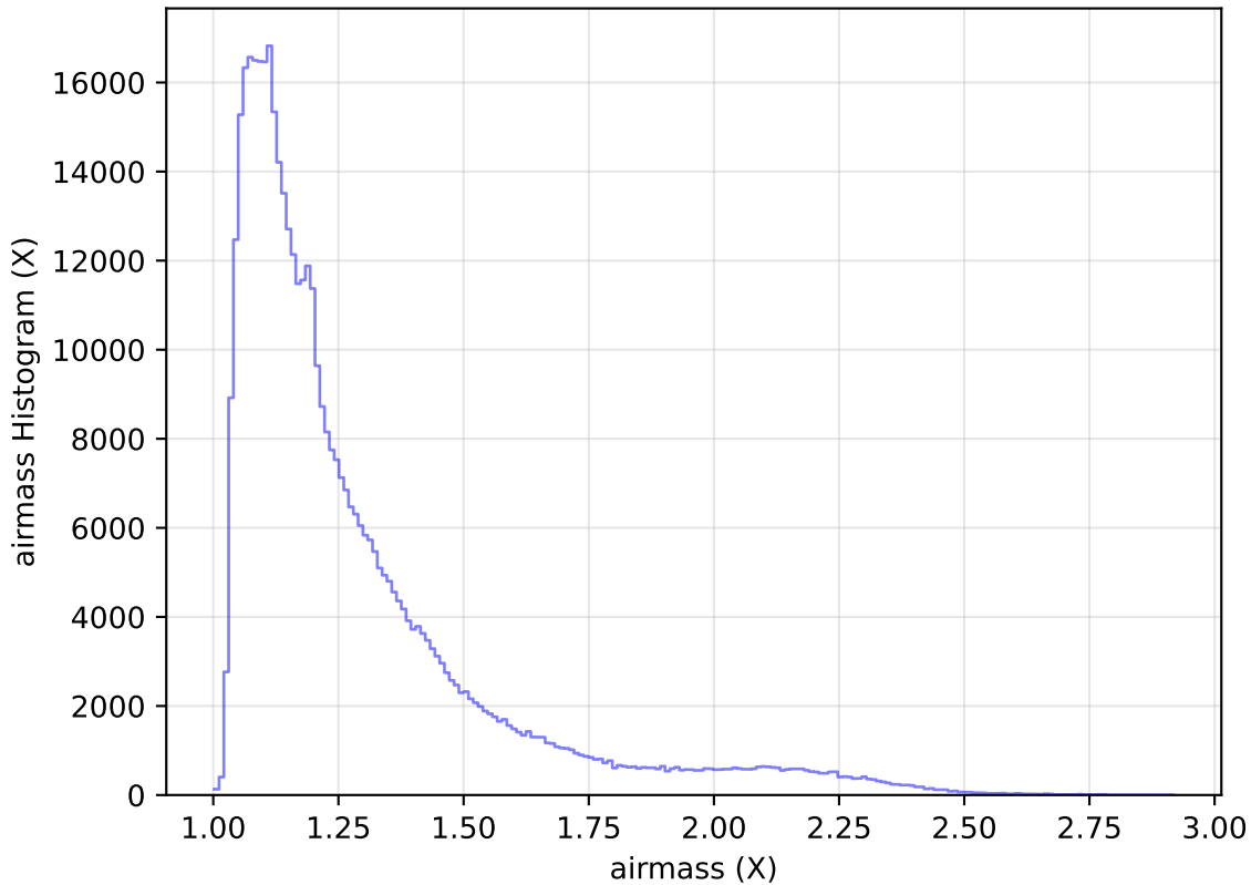
internal_u_expt30_nscale1.1v3.4_10yrs All sky r band: airmass Histogram
