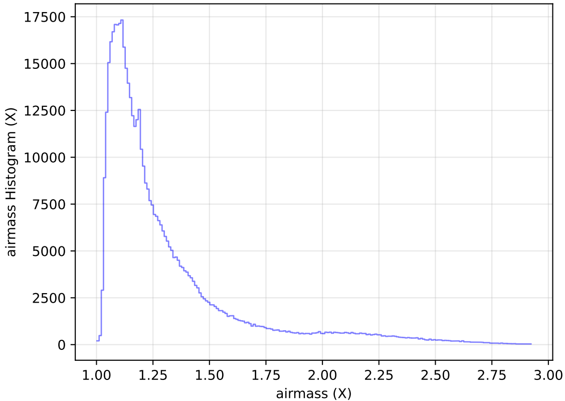
internal_u_expt30_nscale1.1v3.4_10yrs All sky i band: airmass Histogram
