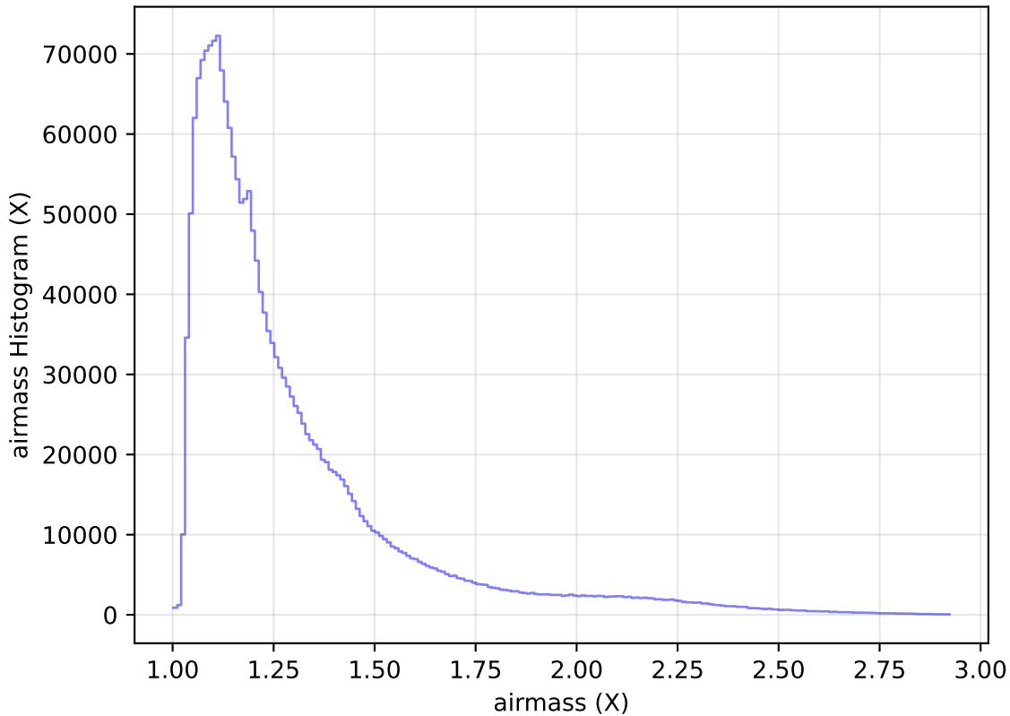
internal_u_expt30_nscale1.1v3.4_10yrs All sky all bands: airmass Histogram
