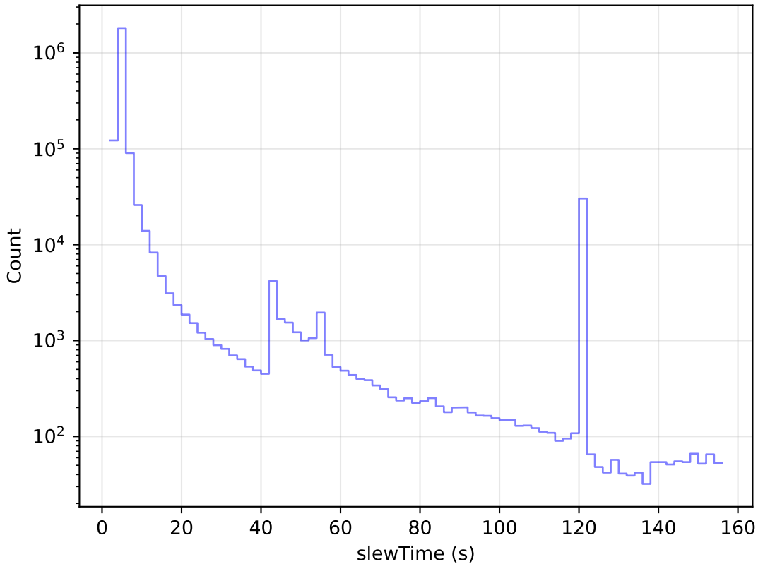
internal_u_expt30_nscale1.1v3.4_10yrs All visits: Slew Time Histogram
