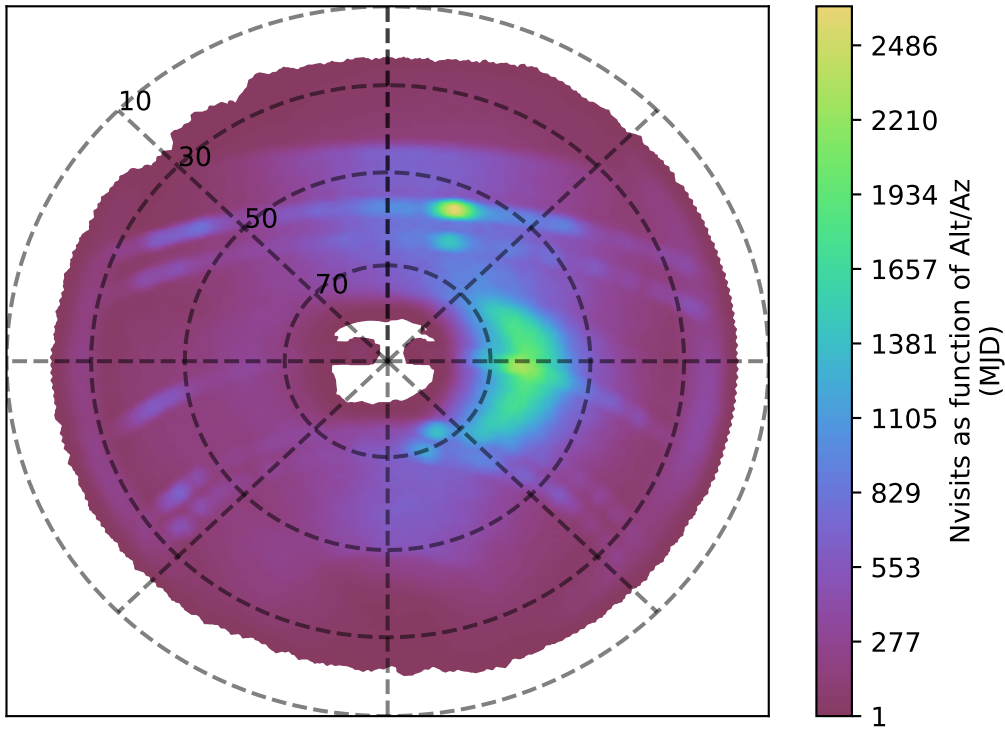
internal_u_expt30_nscale1.1v3.4_10yrs z band: Nvisits as function of Alt/Az
