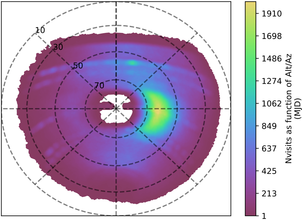
internal_u_expt30_nscale1.1v3.4_10yrs y band: Nvisits as function of Alt/Az
