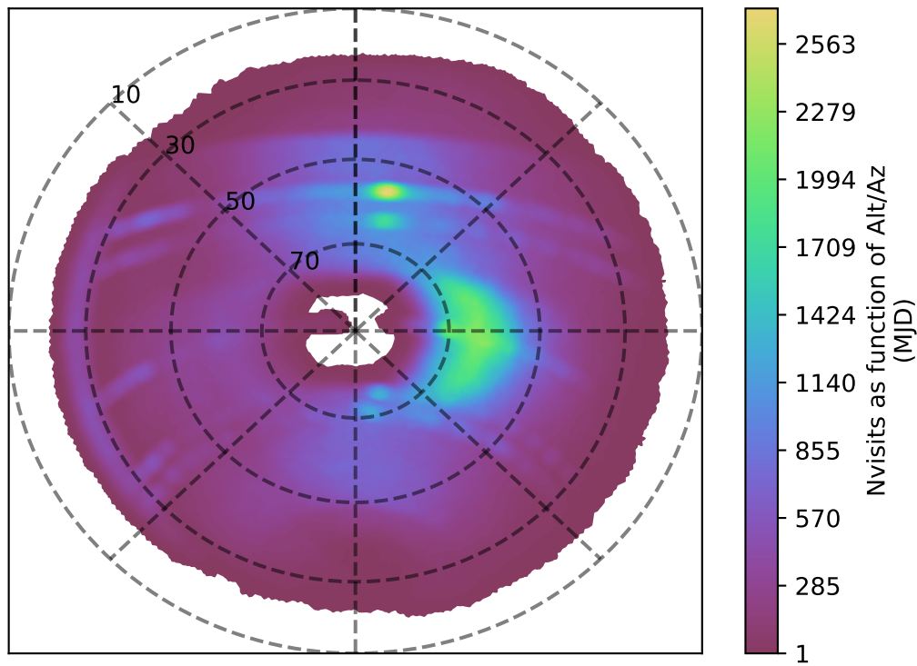
internal_u_expt30_nscale1.1v3.4_10yrs r band: Nvisits as function of Alt/Az
