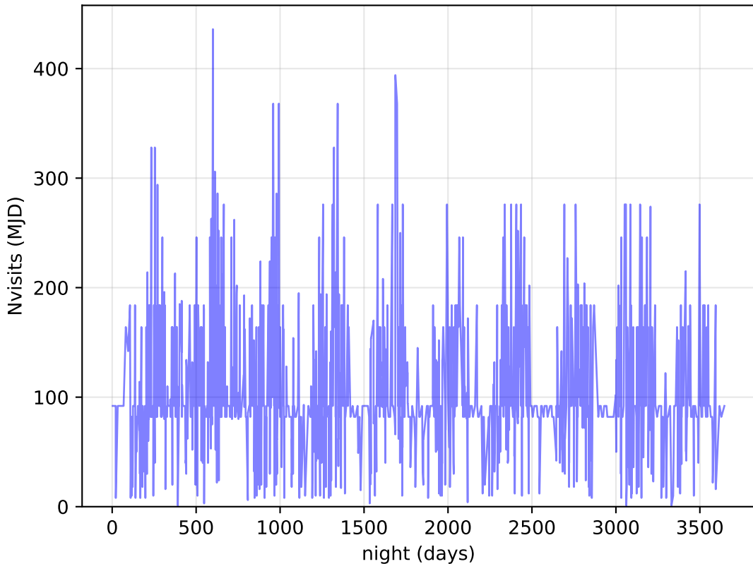
internal_u_expt30_nscale1.1v3.4_10yrs DDF: Nvisits
