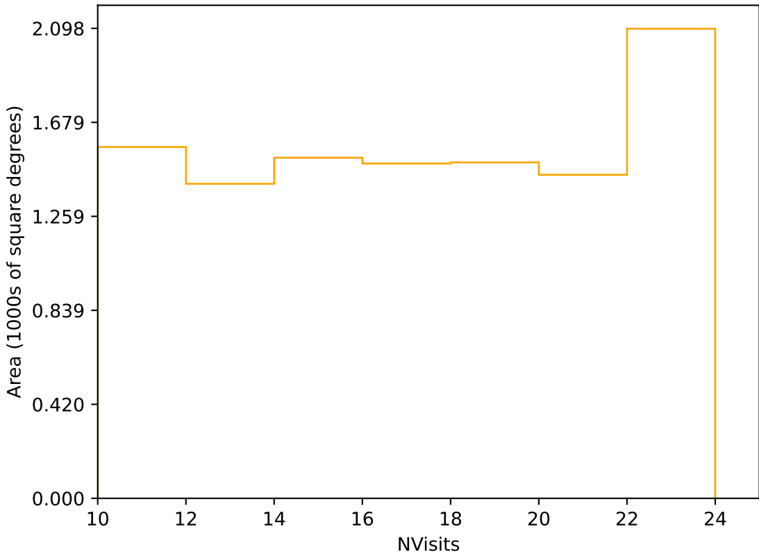
internal_u_expt30_nscale1.1v3.4_10yrs Yr 3-4 r band: NVisits
