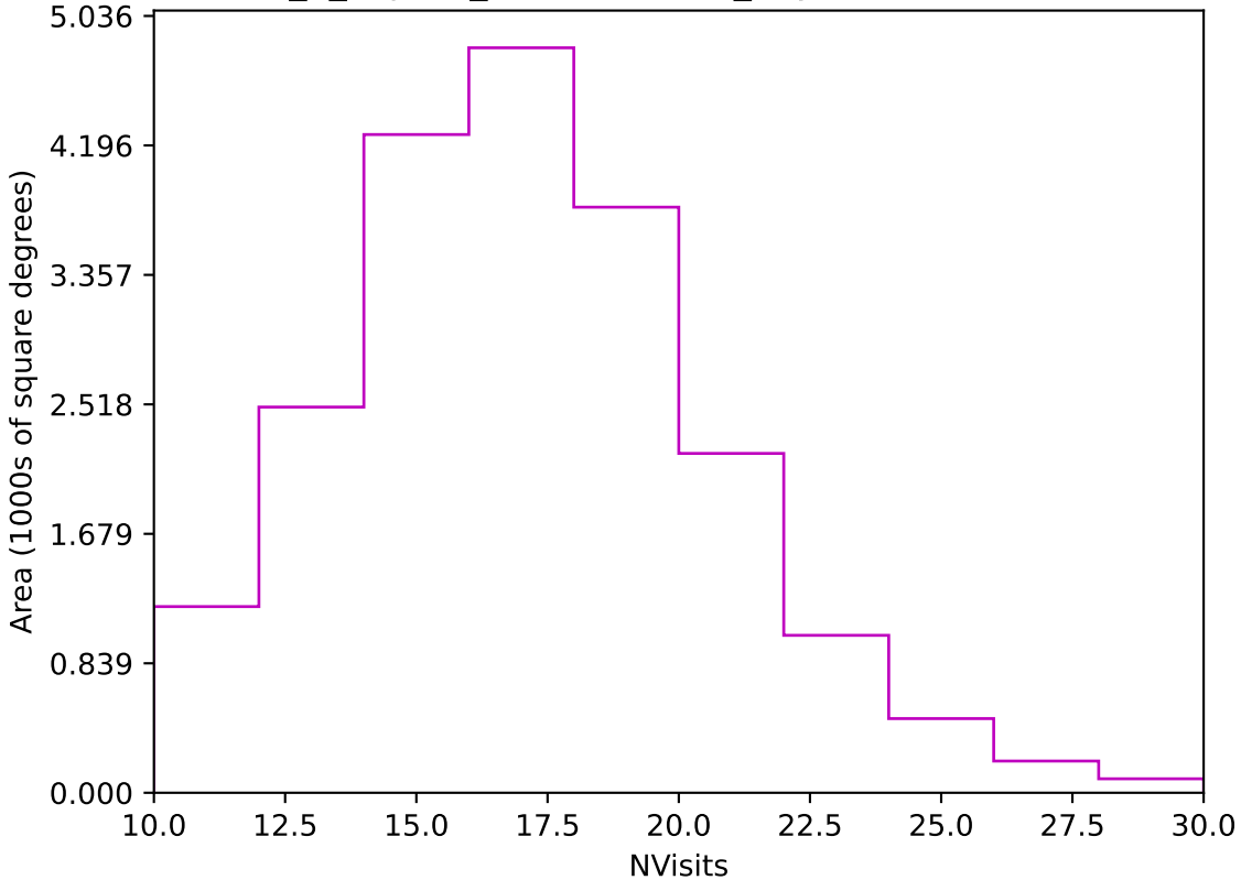
internal_u_expt30_nscale1.1v3.4_10yrs Yr 1 z band: NVisits
