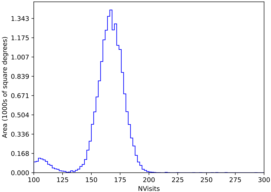
internal_u_expt30_nscale1.1v3.4_10yrs WFD y band: NVisits
