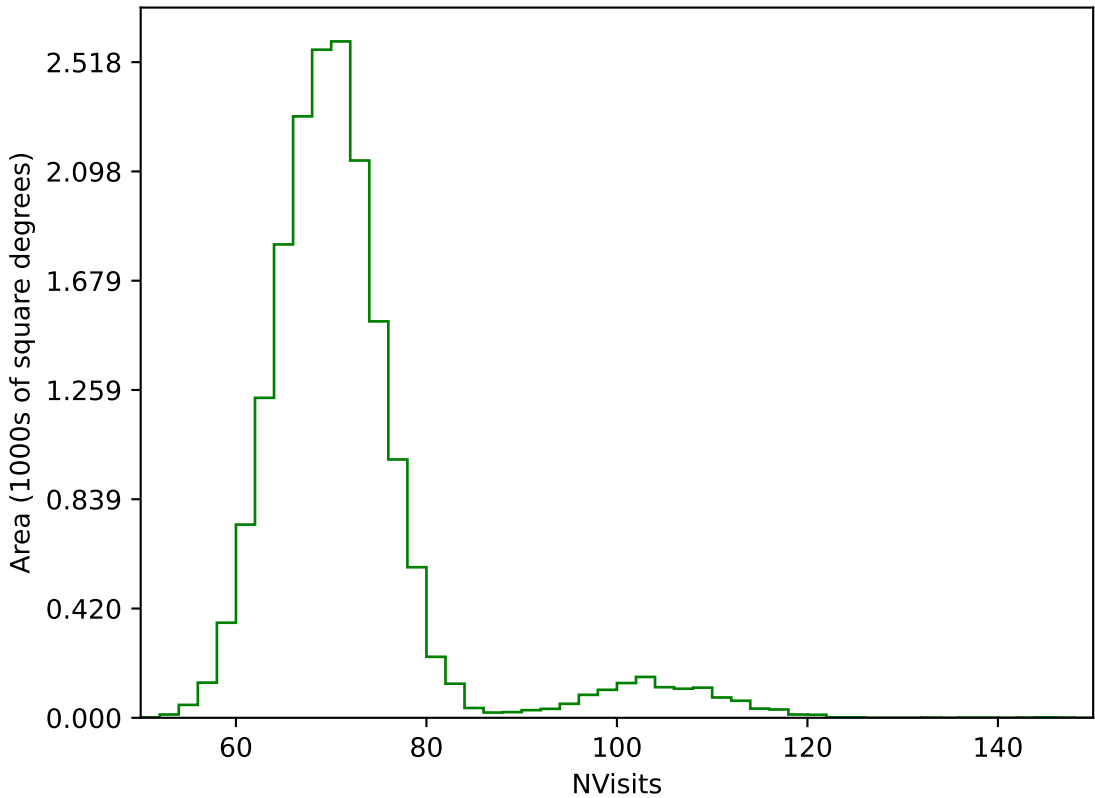
internal_u_expt30_nscale1.1v3.4_10yrs WFD g band: NVisits
