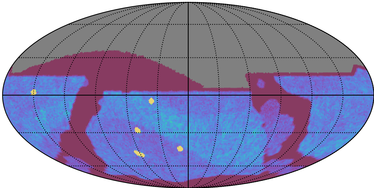
internal_u_expt30_nscale1.1v3.4_10yrs All sky z band: NVisits
