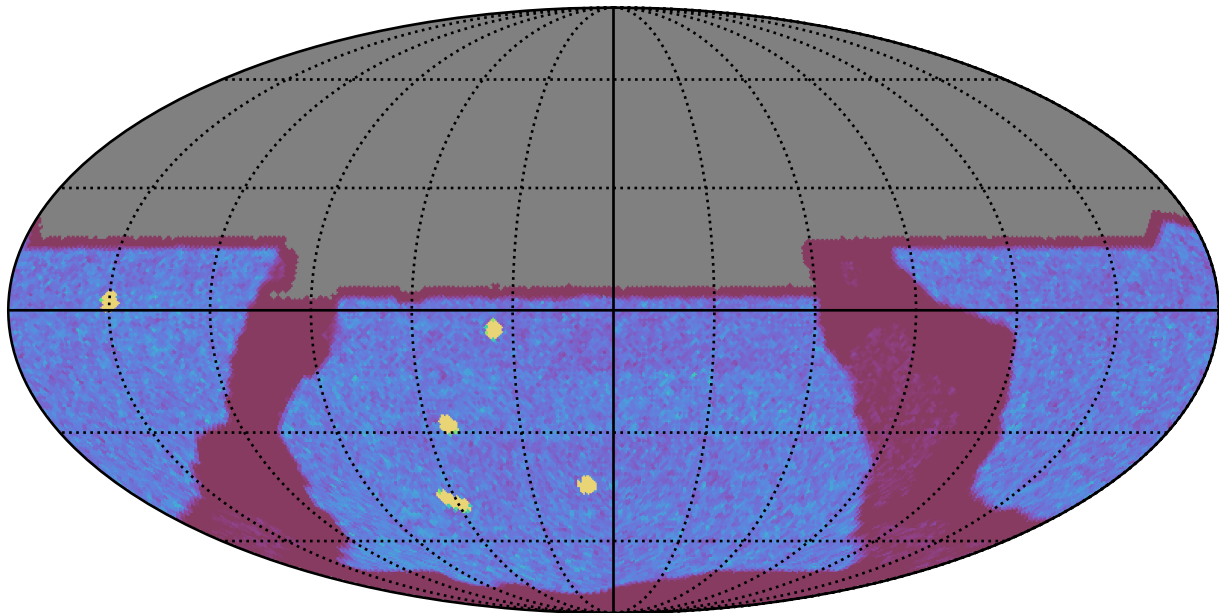
internal_u_expt30_nscale1.1v3.4_10yrs All sky y band: NVisits
