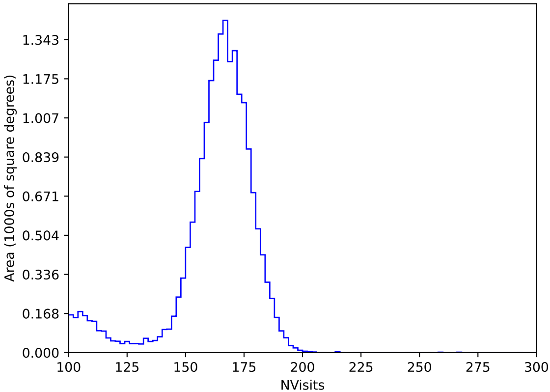
internal_u_expt30_nscale1.1v3.4_10yrs All sky y band: NVisits
