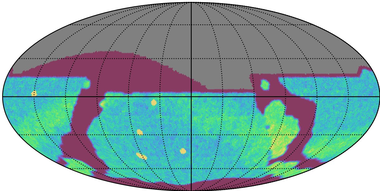
internal_u_expt30_nscale1.1v3.4_10yrs All sky r band: NVisits
