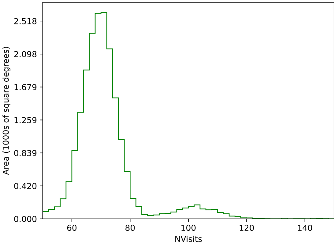
internal_u_expt30_nscale1.1v3.4_10yrs All sky g band: NVisits
