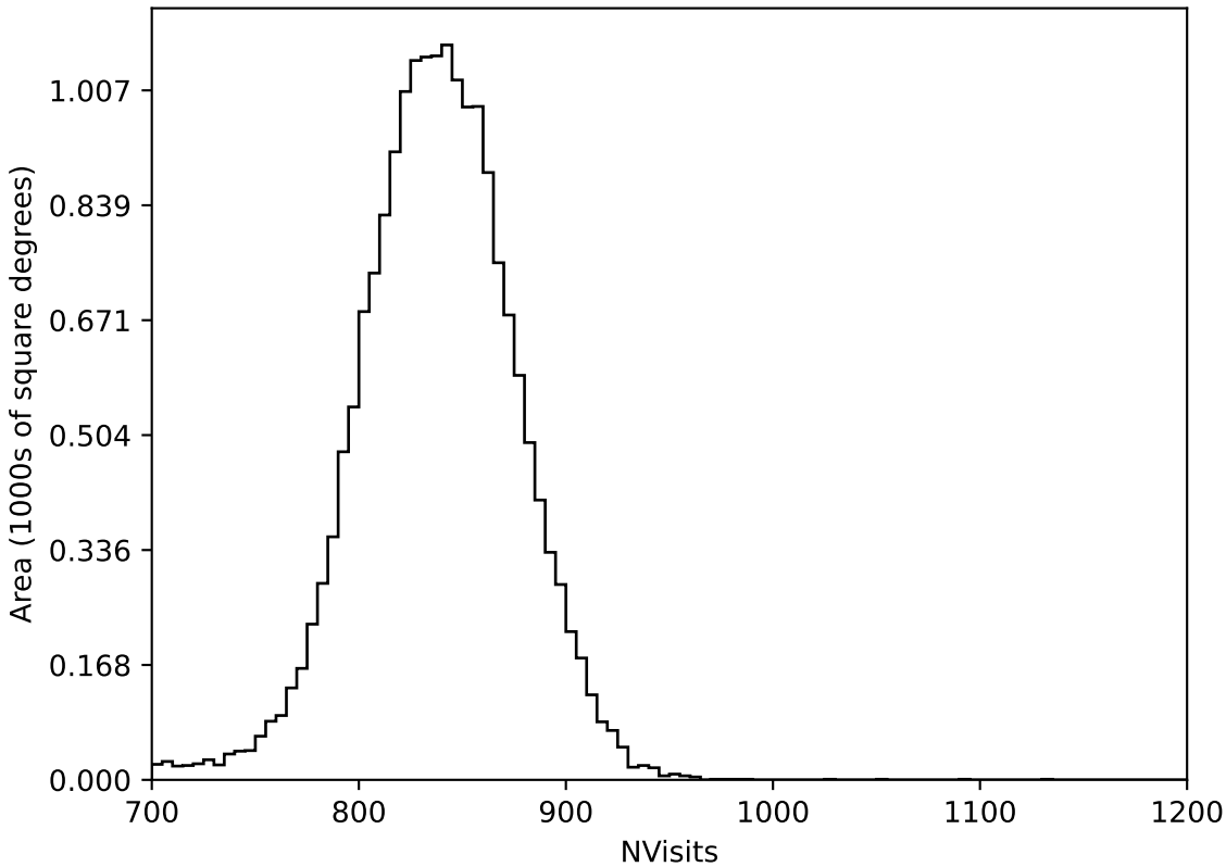
internal_u_expt30_nscale1.1v3.4_10yrs All sky all bands: NVisits
