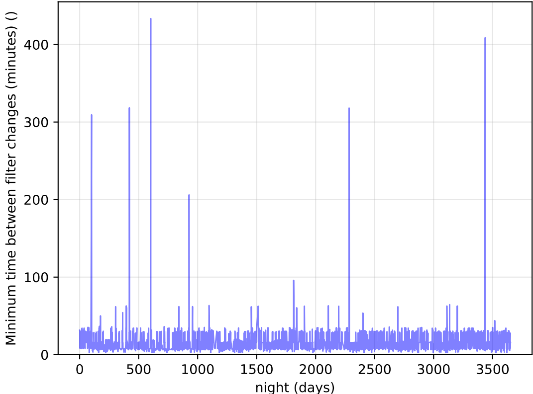
internal_u_expt30_nscale1.1v3.4_10yrs Per Night: Minimum time between filter changes (minutes)
