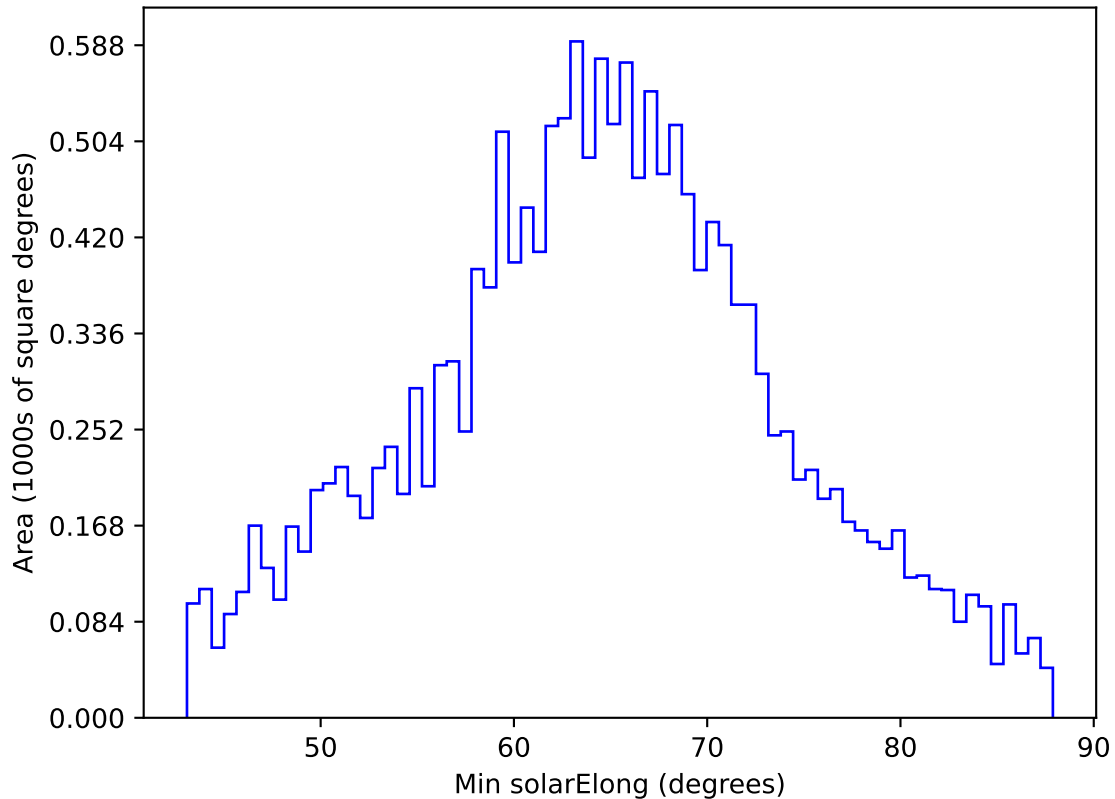
internal_u_expt30_nscale1.1v3.4_10yrs WFD y band: Min solarElong
