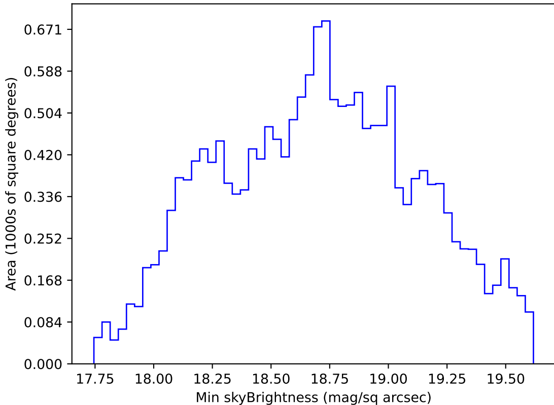
internal_u_expt30_nscale1.1v3.4_10yrs WFD r band: Min skyBrightness
