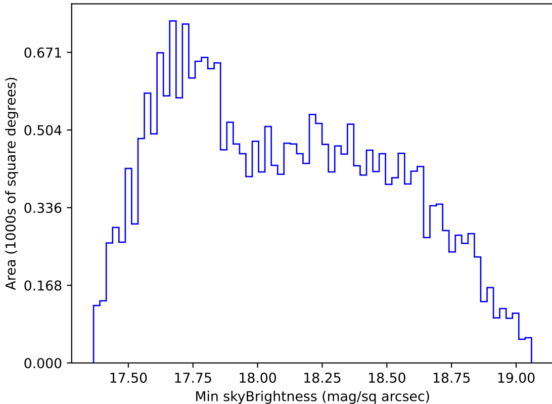
internal_u_expt30_nscale1.1v3.4_10yrs All sky i band: Min skyBrightness
