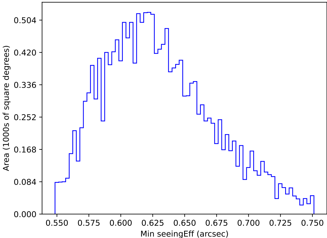
internal_u_expt30_nscale1.1v3.4_10yrs WFD y band: Min seeingEff
