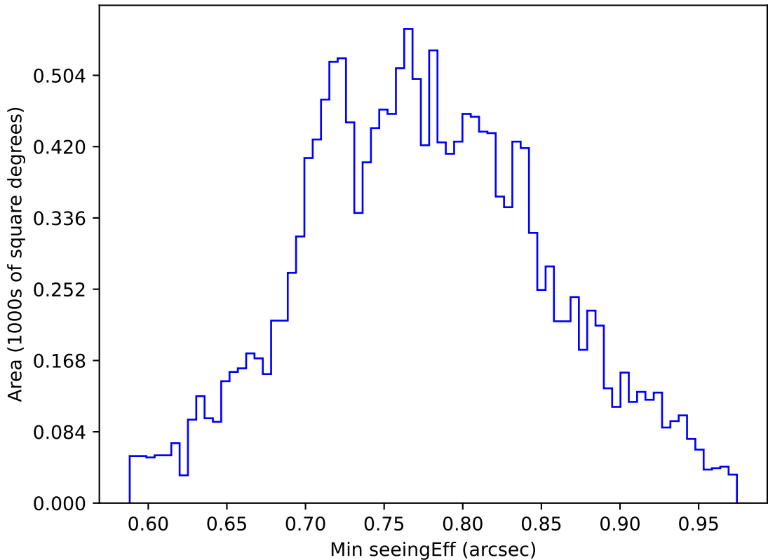
internal_u_expt30_nscale1.1v3.4_10yrs WFD u band: Min seeingEff
