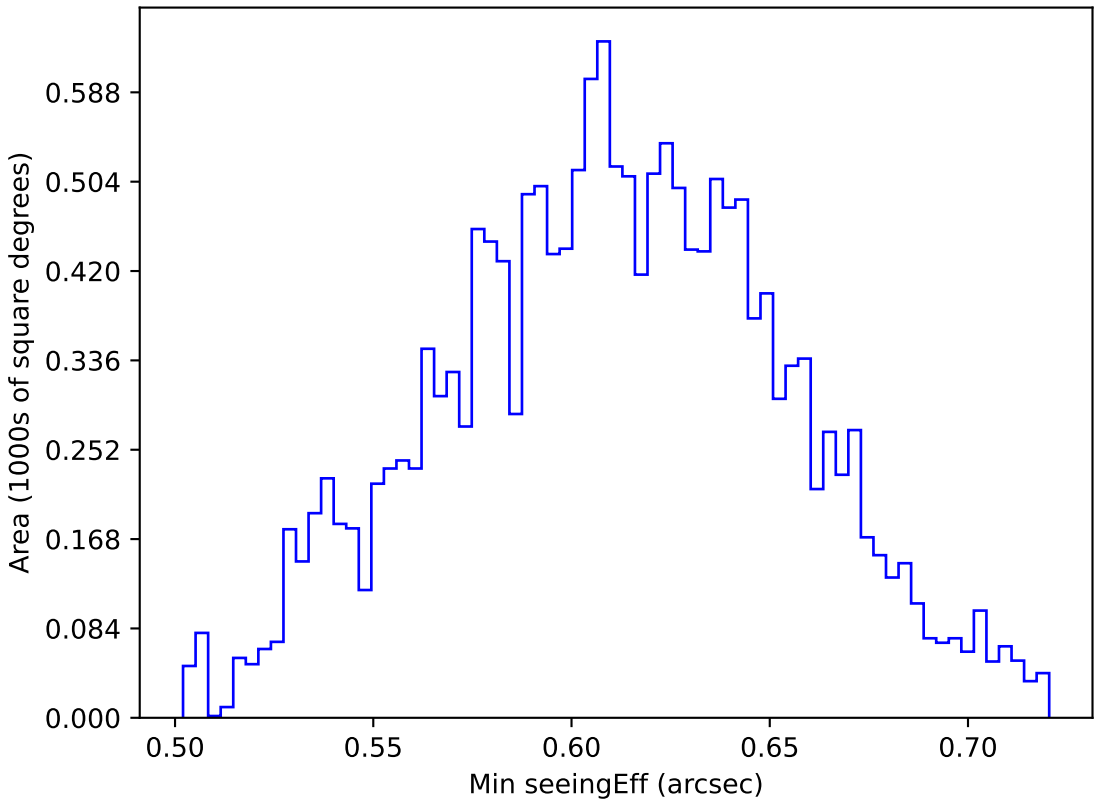
internal_u_expt30_nscale1.1v3.4_10yrs WFD r band: Min seeingEff
