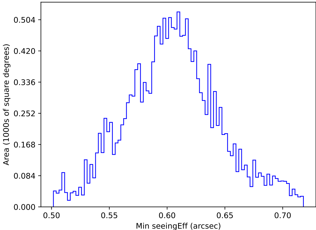
internal_u_expt30_nscale1.1v3.4_10yrs WFD i band: Min seeingEff
