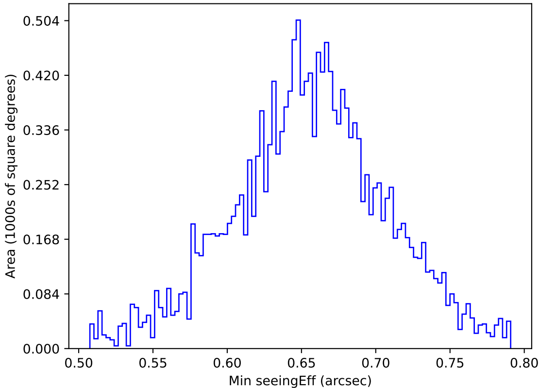
internal_u_expt30_nscale1.1v3.4_10yrs WFD g band: Min seeingEff
