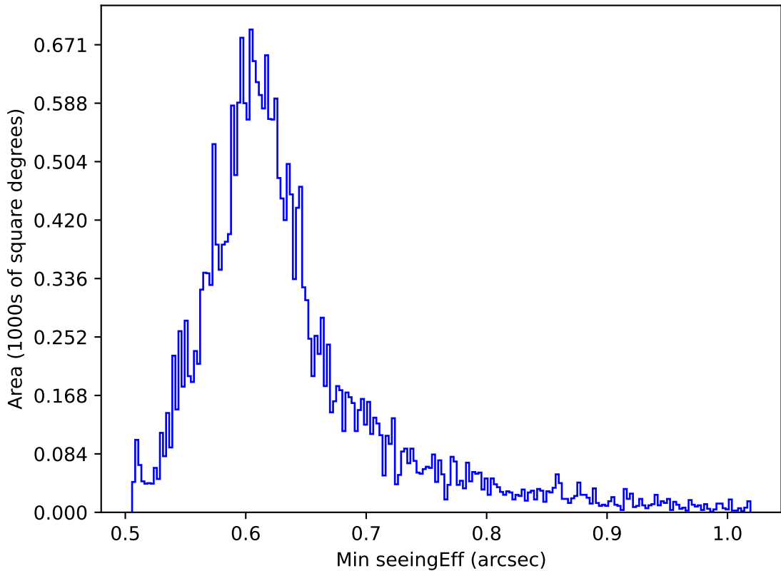
internal_u_expt30_nscale1.1v3.4_10yrs All sky i band: Min seeingEff
