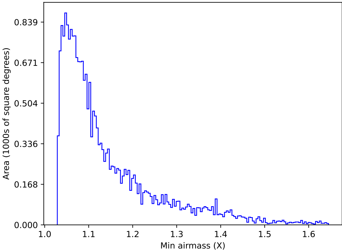
internal_u_expt30_nscale1.1v3.4_10yrs Yr 1 u band: Min airmass
