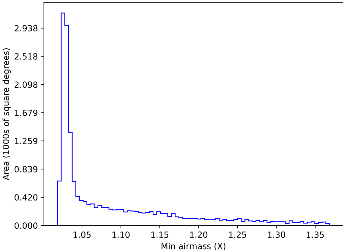
internal_u_expt30_nscale1.1v3.4_10yrs WFD z band: Min airmass
