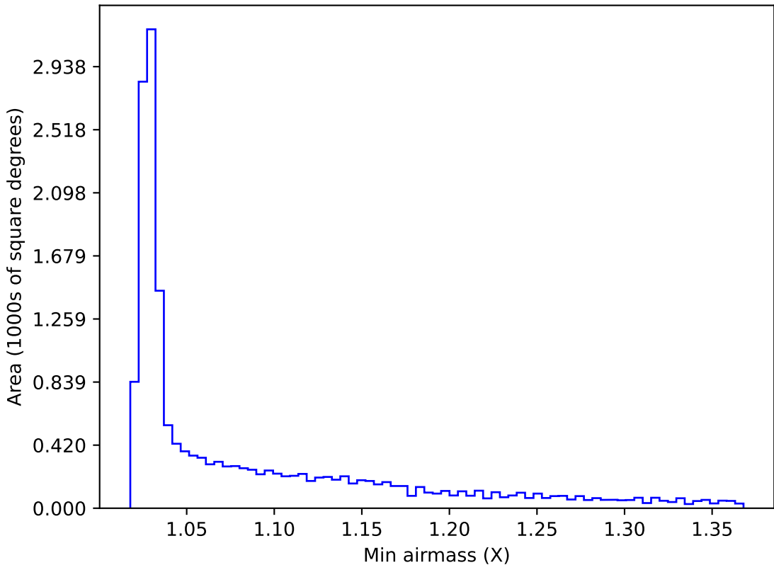
internal_u_expt30_nscale1.1v3.4_10yrs WFD i band: Min airmass
