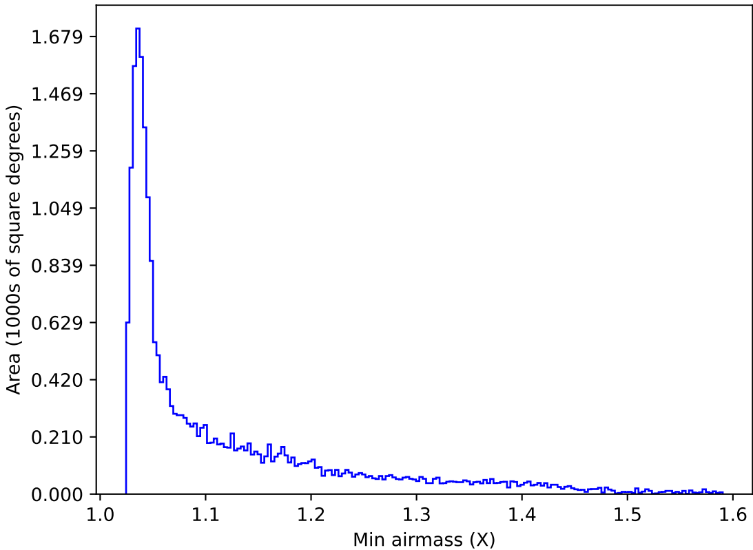
internal_u_expt30_nscale1.1v3.4_10yrs All sky u band: Min airmass
