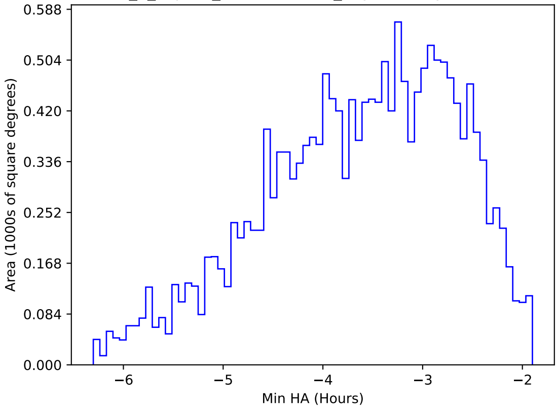
internal_u_expt30_nscale1.1v3.4_10yrs WFD y band: Min HA
